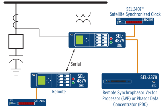
Use real-time control in the SEL-487V for simple applications and in the SEL-3378 for more complex applications.
