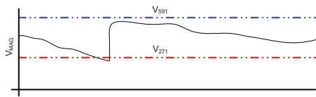
Figure 1. Voltage Control Deadband Characteristics
